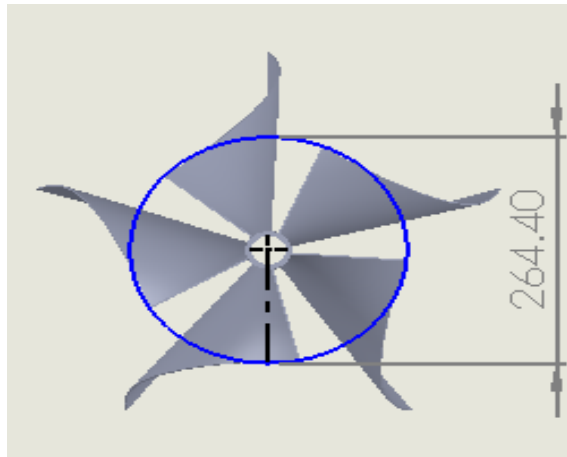
Gambar 2. Diameter 2 (D2) sudu turbin vortex
